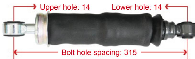
H73-5001450E Liuqi H7 Front Air Spring
