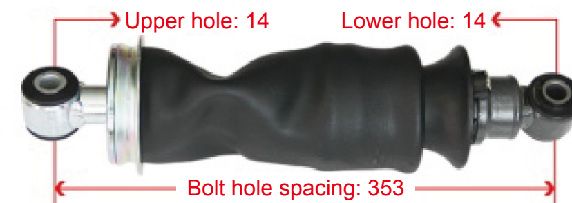
H735001550 Liuqi H7 Rear Air Spring
